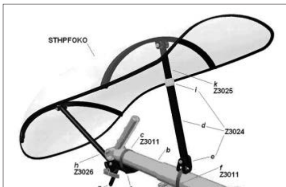
Length 100 cm • Width 55 cm • material: transparent plastic (PETG) • disc 1200 g • Quickmount-adaptor 985 g
